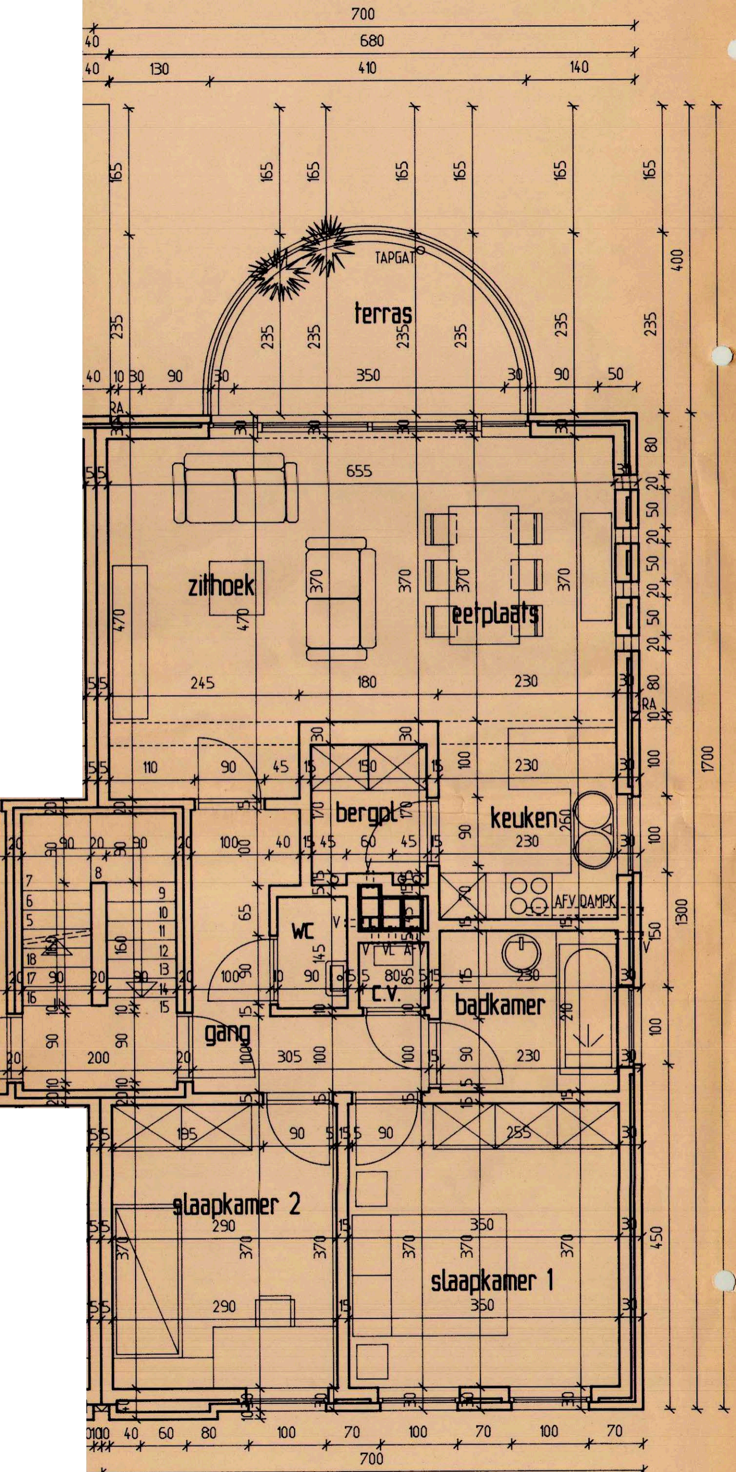
EPINGSPLAN
