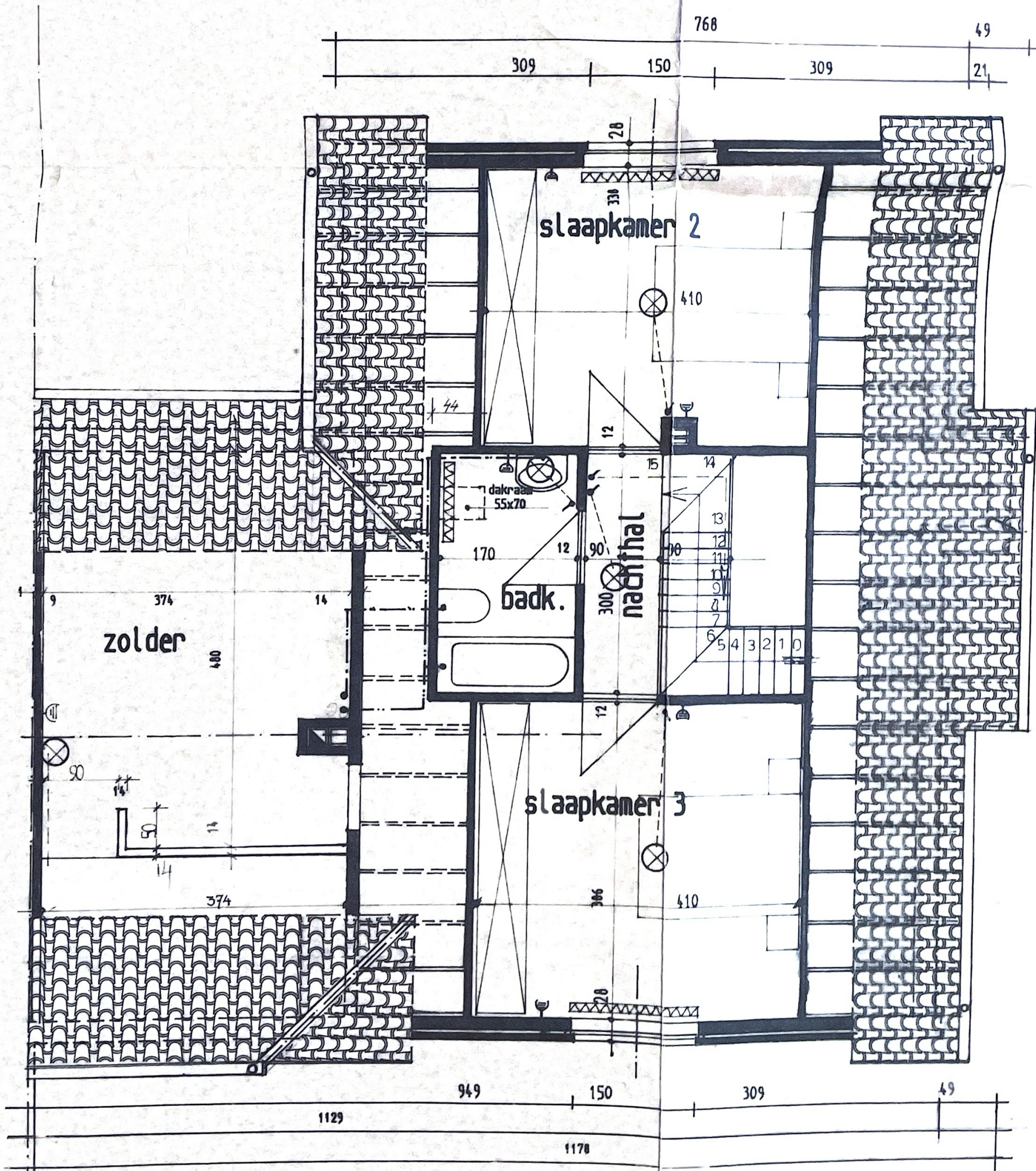
PLAN DAKVERDIEPING 1/50
